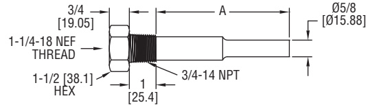
Standard Thermowell
