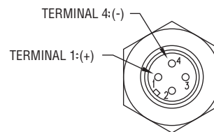
Male-12 Connector
