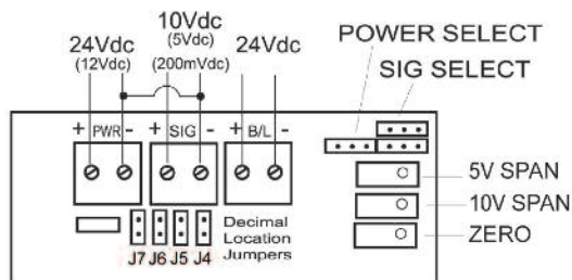
(upper) WIRING
