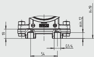
Drawing with mounted adapter (centre distance 54 mm)
